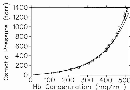
FIGURE 2 Best-fittings to Adair's osmotic pressure data published by Dick ( \square ) (Dick, 1967). The solid curve is the fitting using MSPT ( \chi^2_r = 1.5 ). The long-dashed curve is the fitting using BSPT with r_w fixed at 1.375 Å ( \chi^2_r = 0.18 ). The short-dashed curve is the fitting using BSPT with \delta_{\text{Hb}} and r_w floated ( \chi^2_r = 0.14 ). Results of these fittings are summarized in Table 1.
